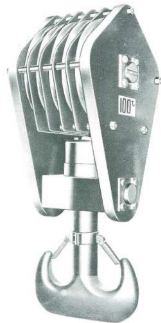
7. 100-ton Hook Block with 5 Sheaves
