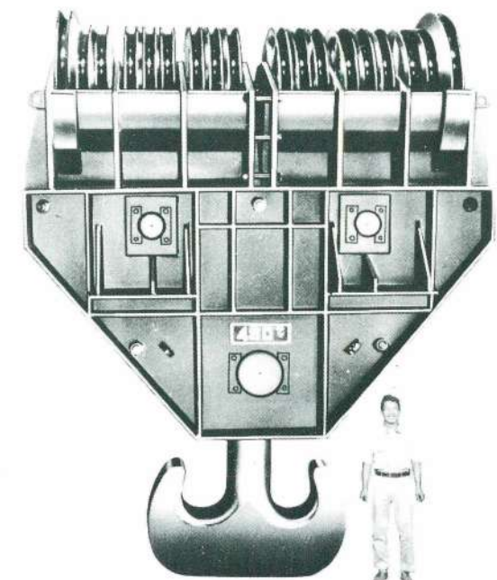
15. 480-ton Hook Block with 18 Sheaves
