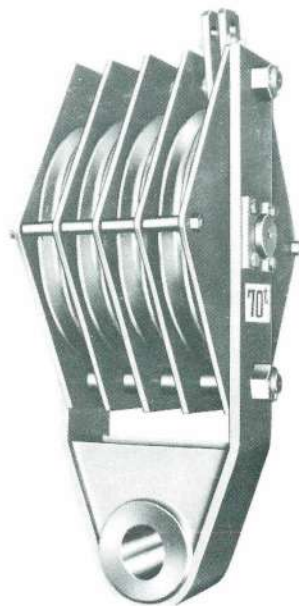
6. 70-ton Hook Block with 4 Sheaves
